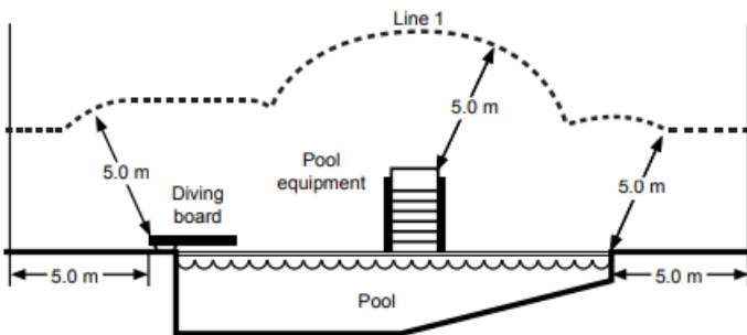
FIGURE 3 - Overhead Conductors Less Than 750 Volts
